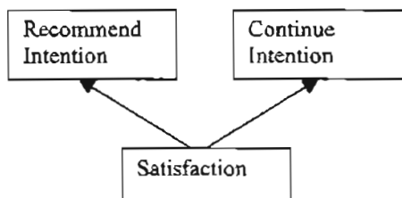
Figure 3 Rival Structural Diagram Accounting for Intercorrelated Measures
